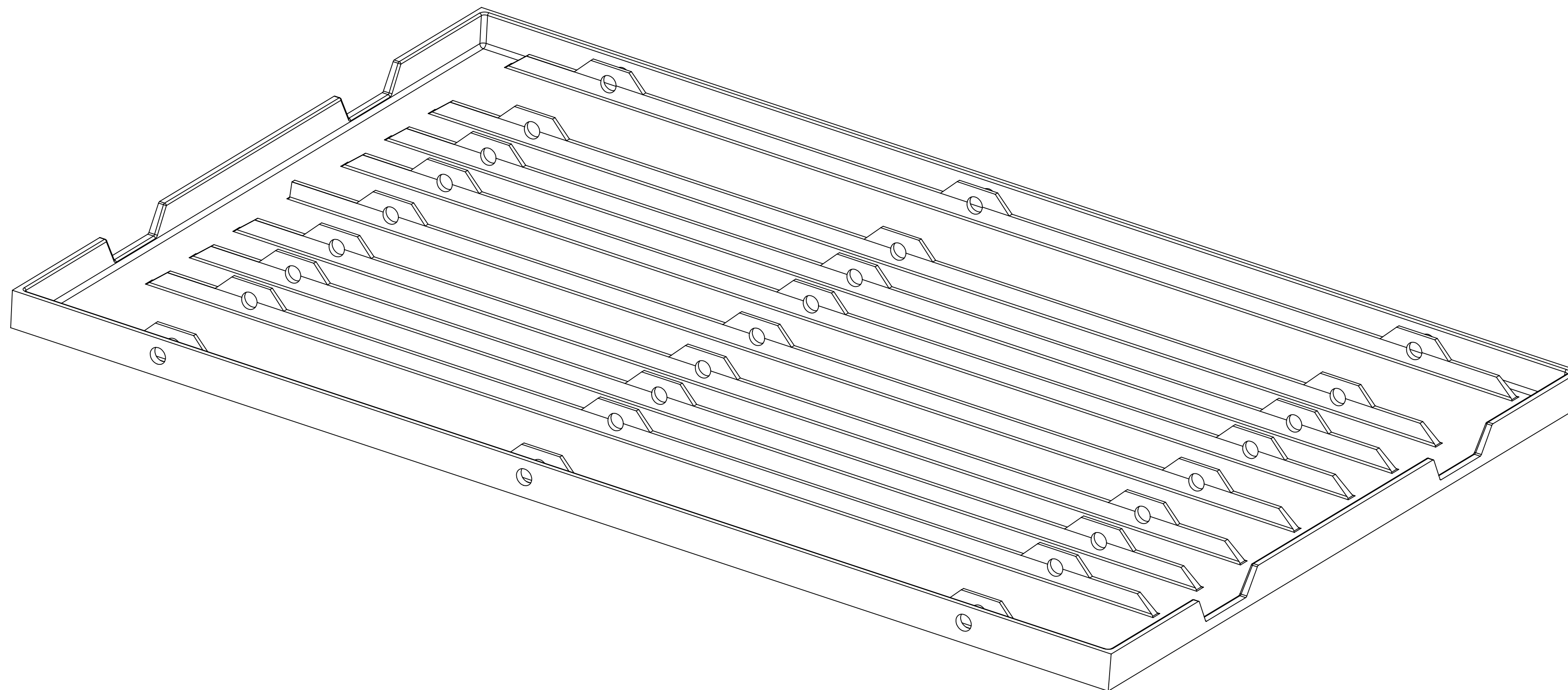
ISOMETRIC VIEW
