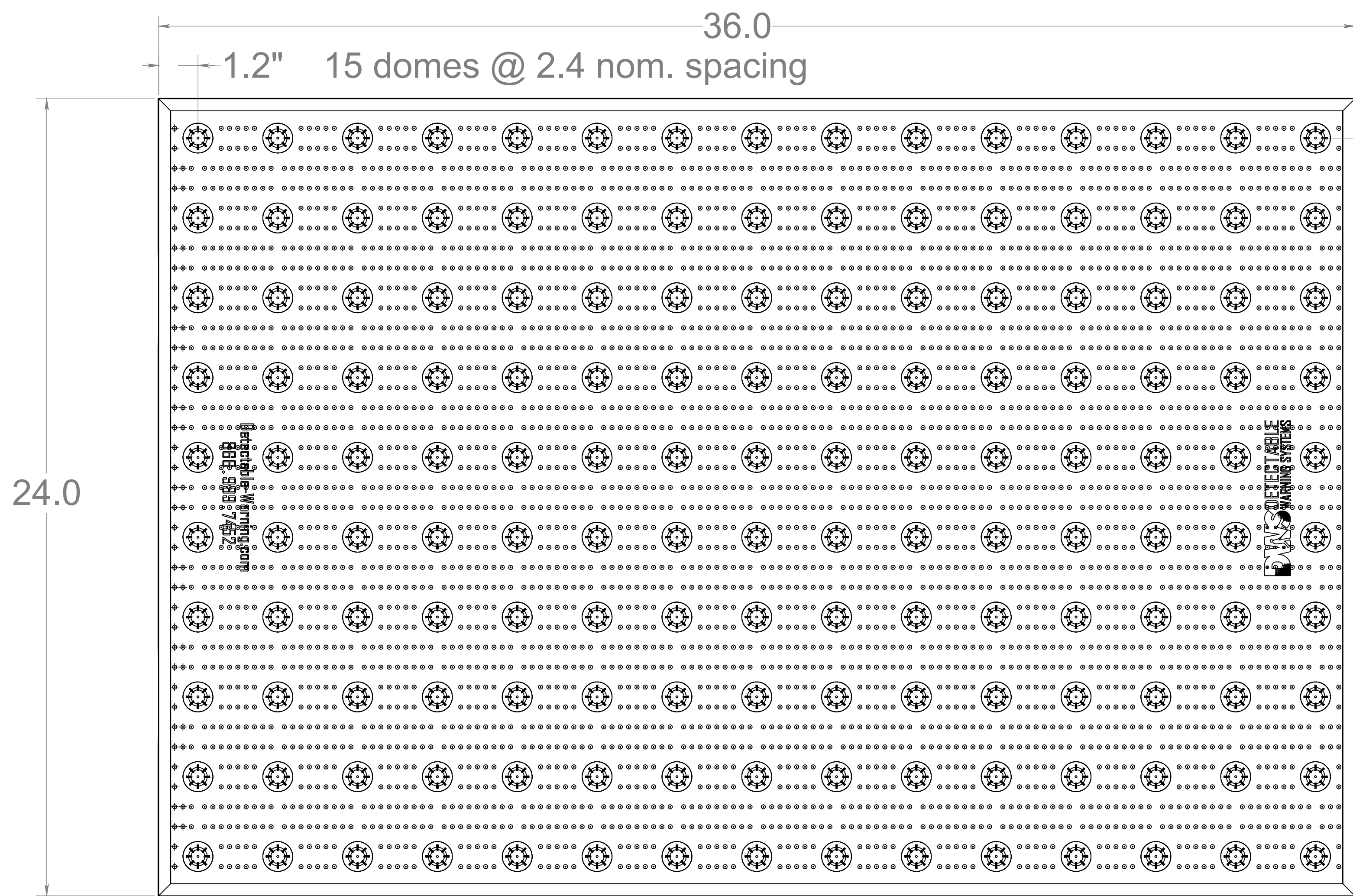
TOP VIEW
