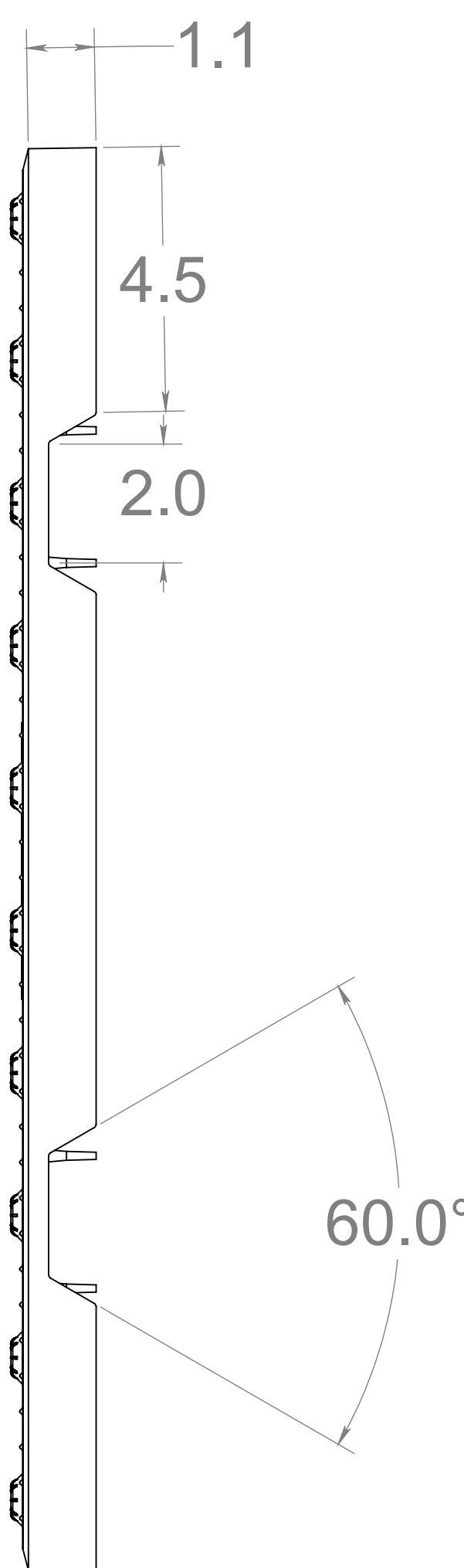
SIDE VIEW
