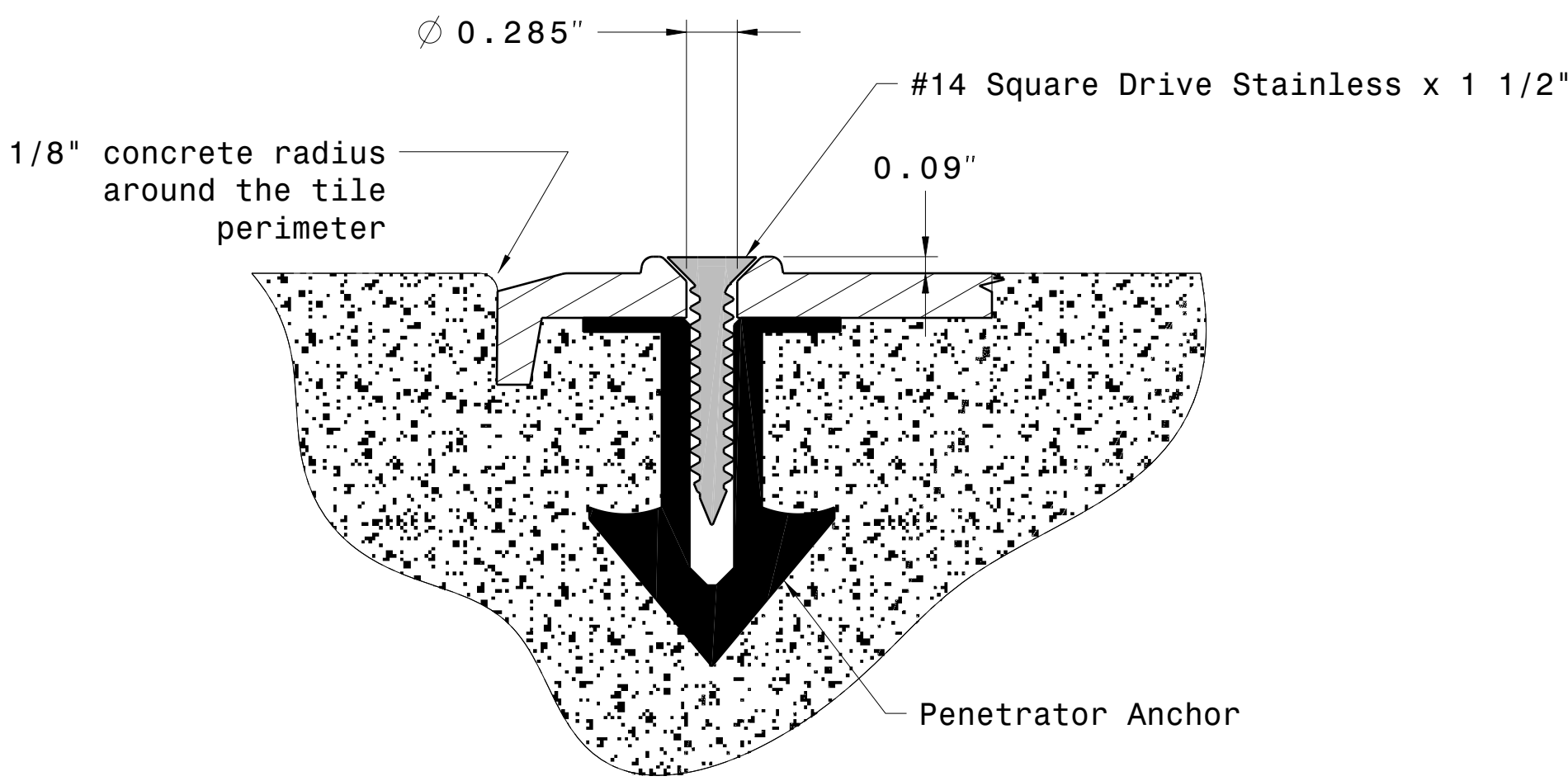
TYPICAL PERIMETER FASTENER DETAIL
