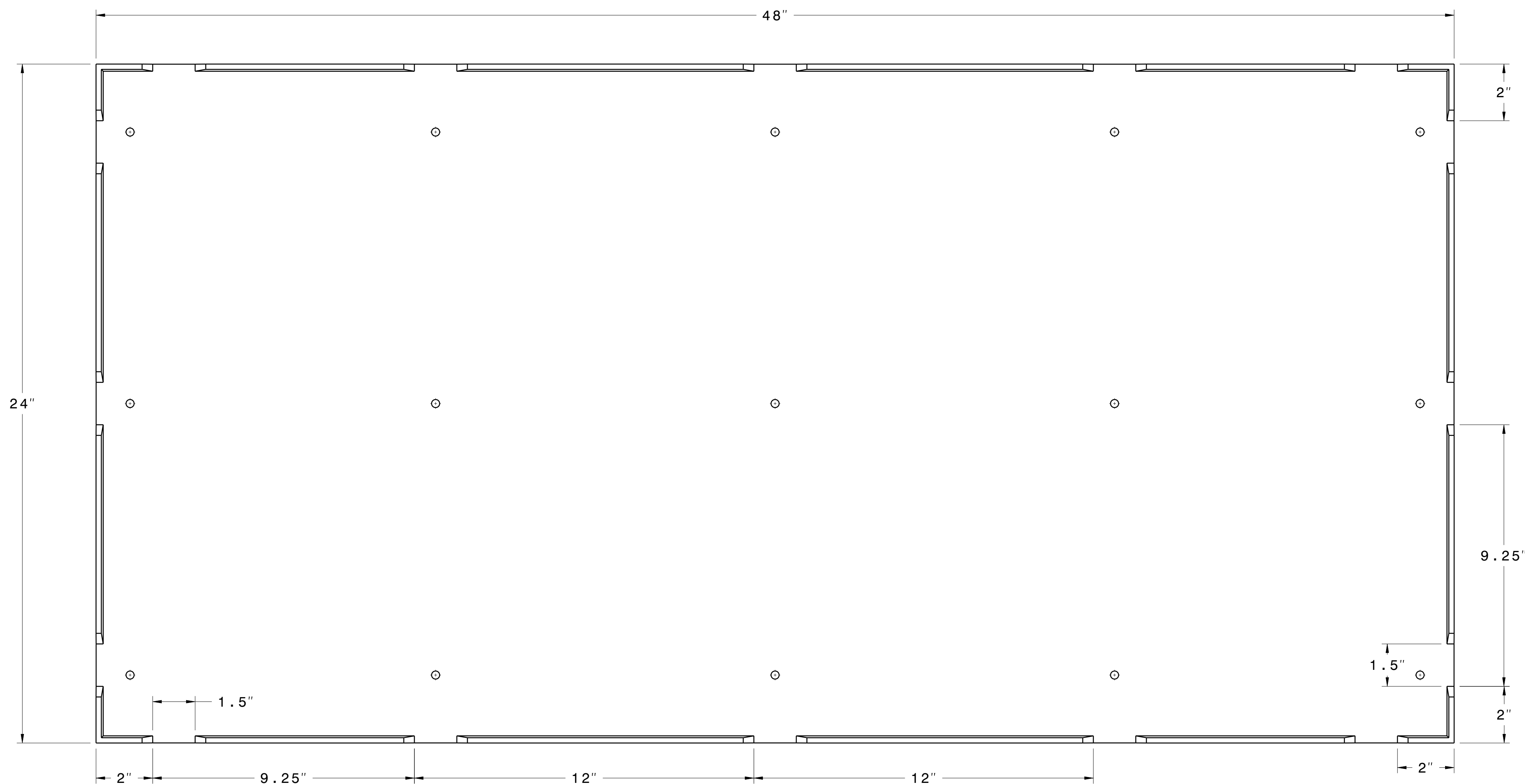
UNDERSIDE VIEW
