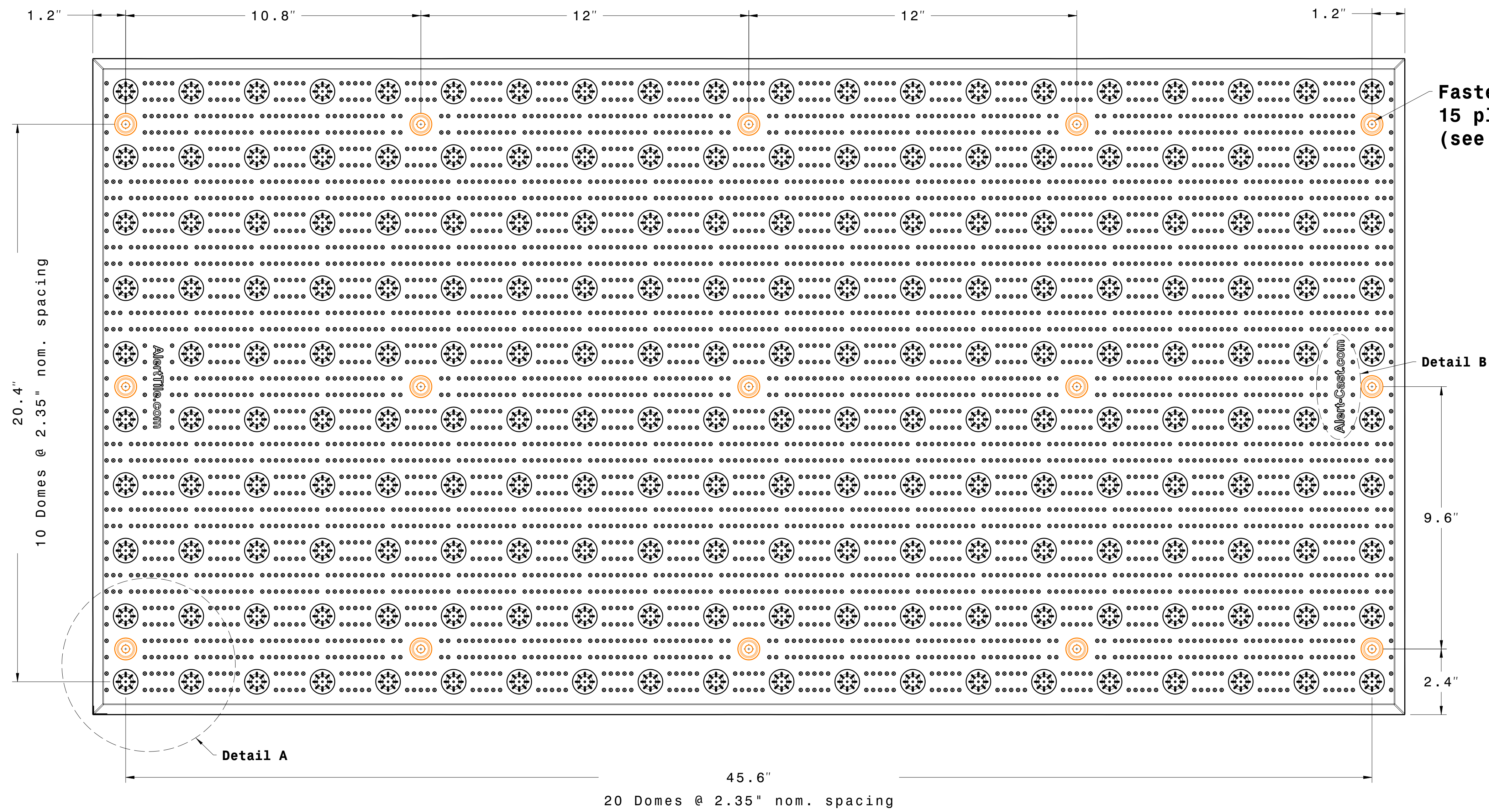
PLAN VIEW
